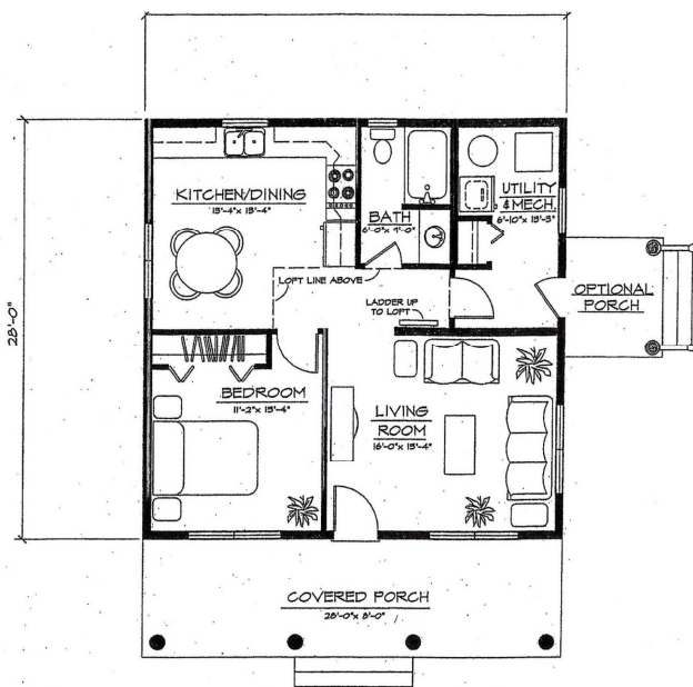
MAIN FLOOR PLAN SCALE: 1/4" = 1'-0"
