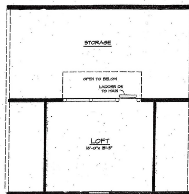
LOFT FLOOR PLAN
