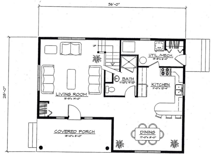
MAIN FLOOR PLAN SCALE: 1/4" = 1'-0"
