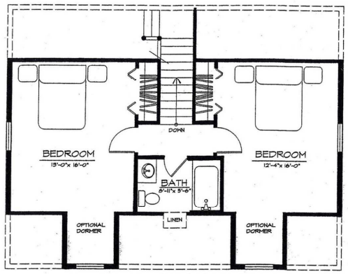
SECOND FLOOR PLAN SCALE: 1/4" = 1'-0"
