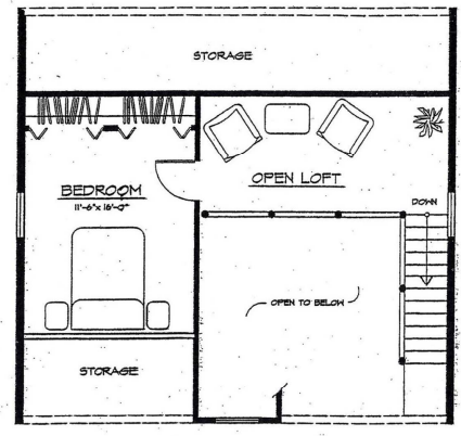
SECOND FLOOR PLAN SCALE: 1/4" = 1'-0"
